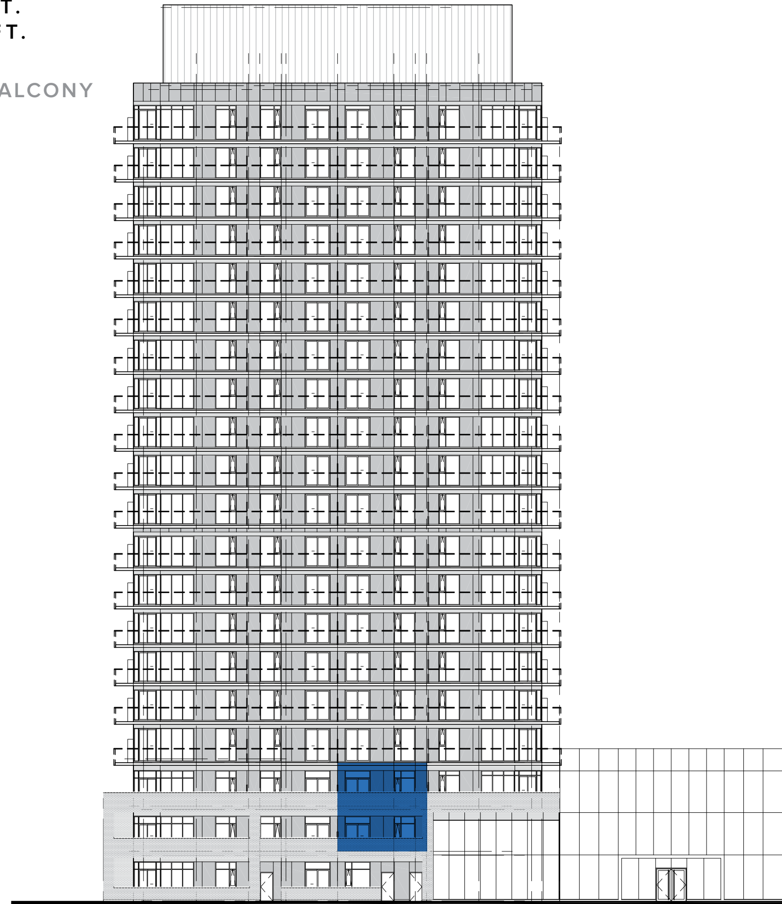
SOUTH ELEVATION
