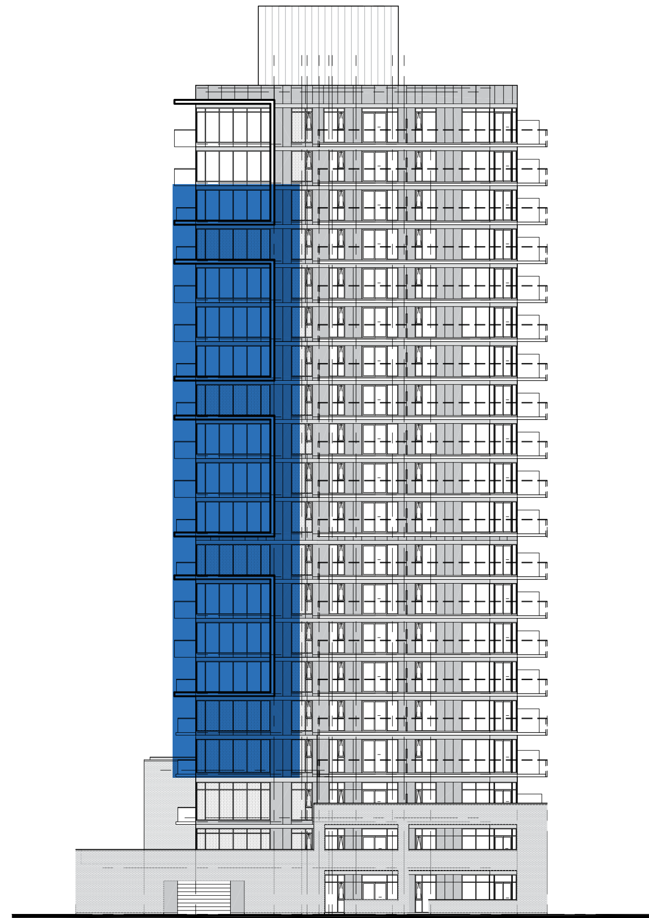
WEST ELEVATION
