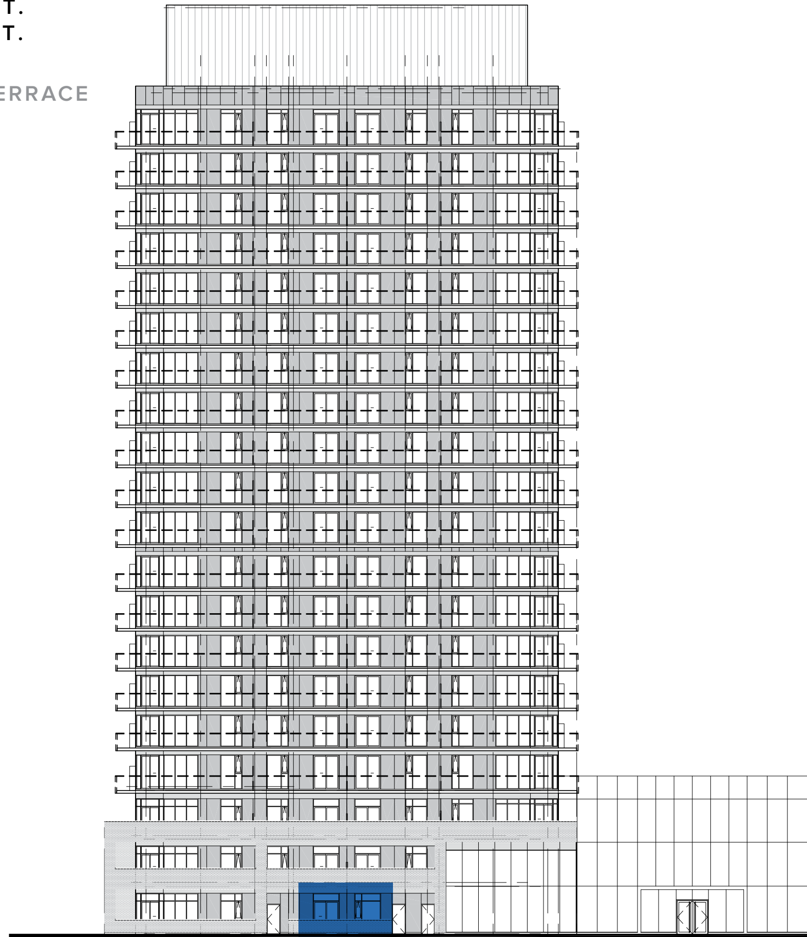
SOUTH ELEVATION
