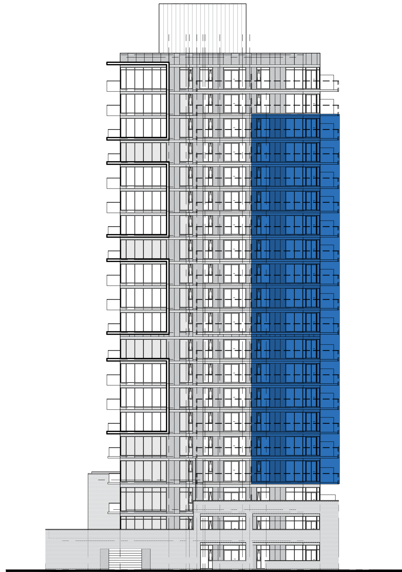
WEST ELEVATION
